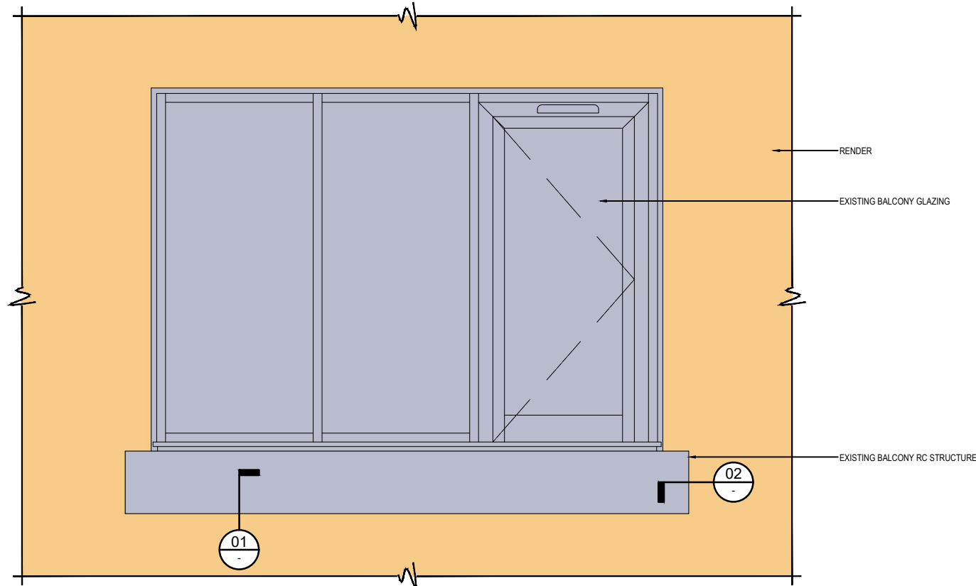
03 PART ELEVATION - RENDER / EXISTING BALCONY
