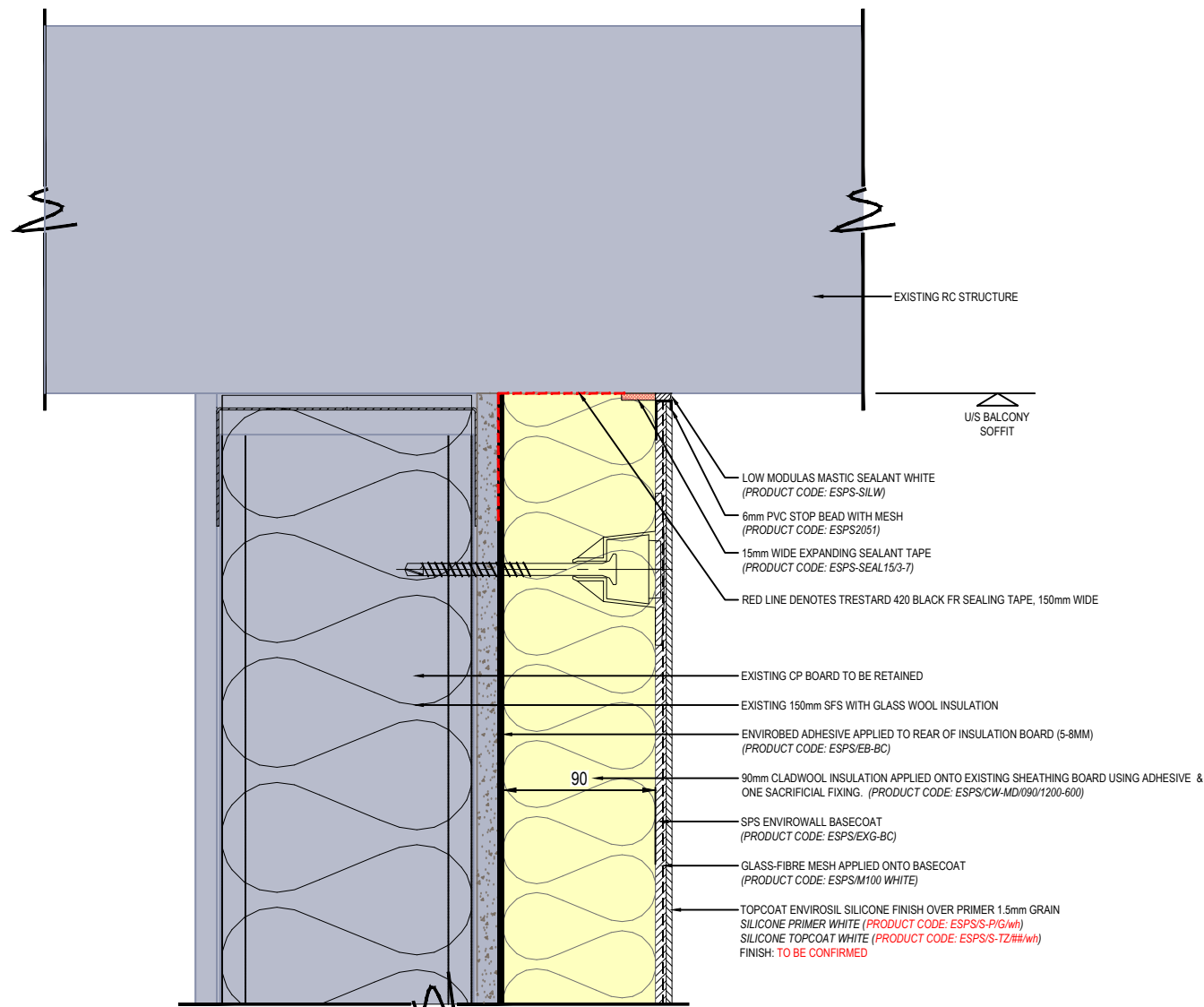
01 CROSS SECTION - RENDER / EXISTING BALCONY STRUCTURE DETAIL
