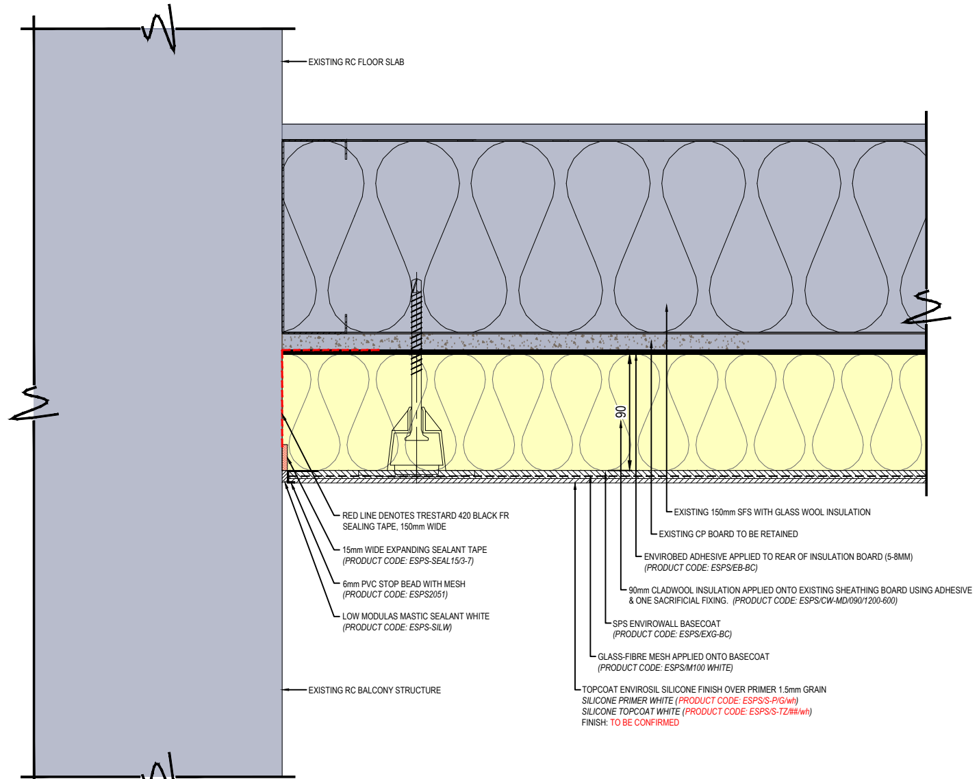
02 PLAN SECTION - RENDER / EXISTING BALCONY STRUCTURE DETAIL
